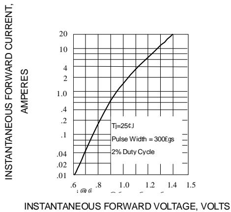
Fig. 2-TYPICAL FORWARD CHARACTERISTICS
